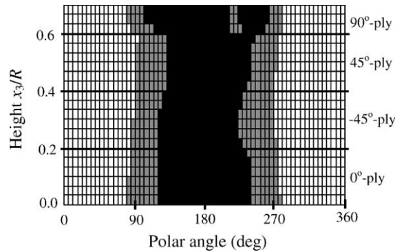
Fig. 13. Map of contact condition after five cycles of unloading and reloading in terms of \epsilon_{11}^\infty upon the first application of bearing force F followed by bypass straining \epsilon_{11}^\infty . The map right before the cycling process is shown in Fig. 11c.
