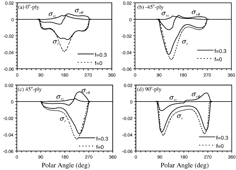
Fig. 9. Variation of the (local) traction components (normalized by E_1 ) with polar angle, at the middle plane of a ply. The loads are F = 0.01\pi E_1 and \varepsilon_{11}^\infty = 0.03 . The cases of f = 0.3 and 0 are studied for comparison. Note that in the case of f = 0 , the tangential components \sigma_{r\theta} and \sigma_{rz} , whose value is zero, are not shown above.
