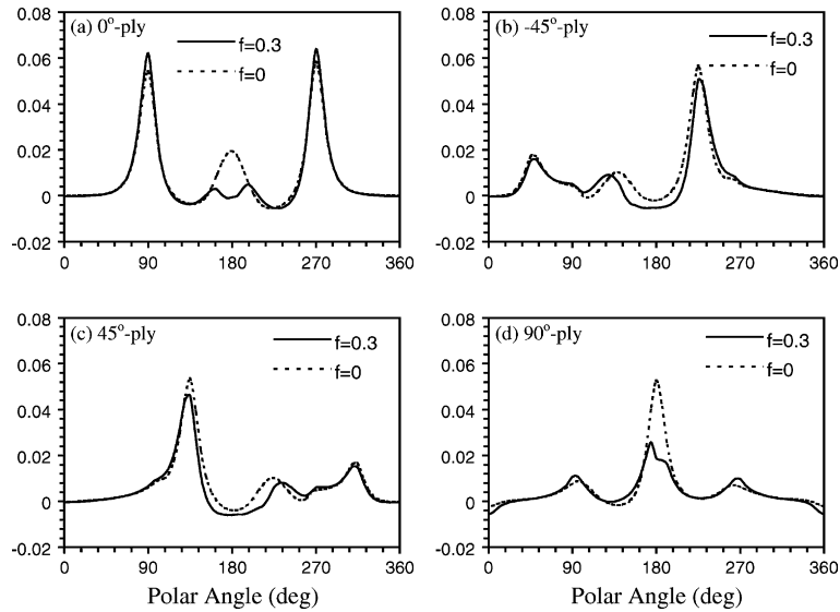
Fig. 6. Variation of the normalized hoop stress, \sigma_{\theta\theta}/E_1 , with polar angle, at the middle plane of a ply. The loads are F = 0.01\pi E_1 and \varepsilon_{11}^\infty = 0 . The cases of f = 0.3 and 0 are compared.
