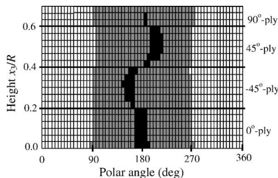
Fig. 4. Contact condition between the composite and pin under e_{11}^\infty = 0 and F = 0.01\pi E_1 , in the case of f = 0.3 (black color—stick contact zone; gray color—slip contact zone; white color—separation zone).
